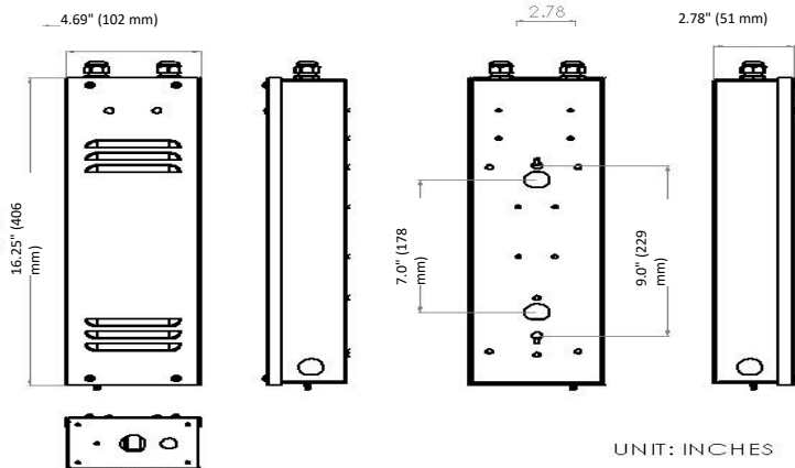
BALLAST BOX (SINGLE or DOUBLE)
