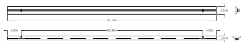
EXTRUDED REFLECTOR
